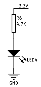
PWR指示灯
